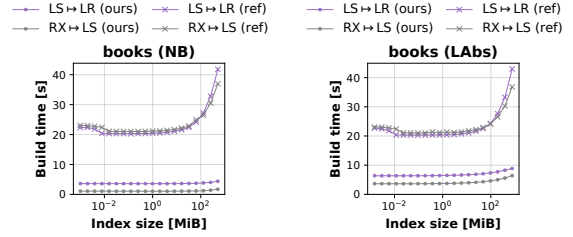
(a) No bounds (b) Local absolute bounds Figure 11: Build times of our implementation (ours) and the reference implementation (ref) with NB and LABs.
